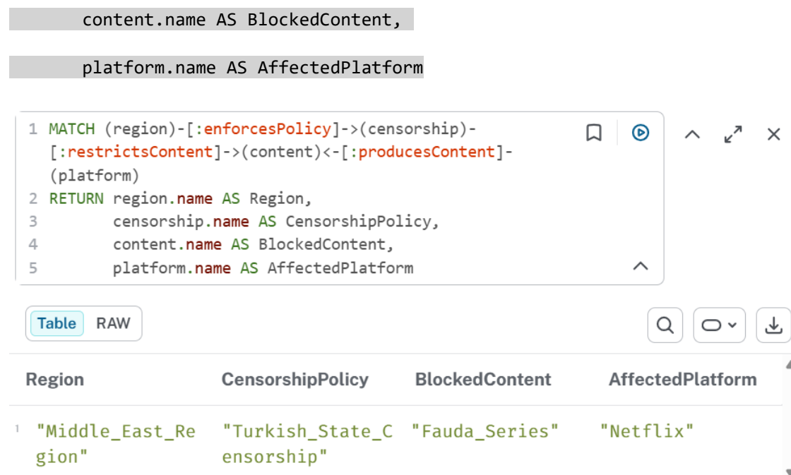
Figure D.4: Gemini four-node traversal identifying regional censorship policies and restricted content.
